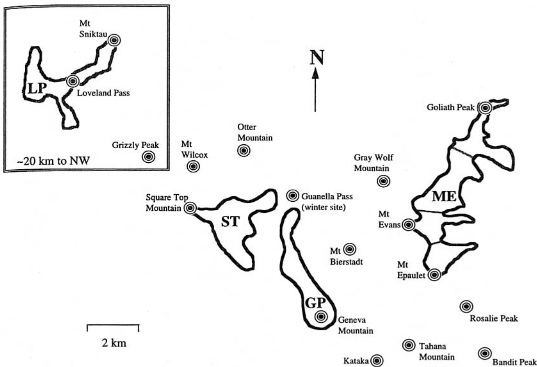
FIGURE 1. Study sites for White-tailed Ptarmigan in Colorado, including Guanella Pass winter site and adjacent mountains that were surveyed less intensively in late summer. ME—Mt. Evans, GP—Guanella Pass, ST—Square Tops, and LP—Loveland Pass. The shaded lines on ME study area indicate the four major drainages used to evaluate philopatry of internal recruits.
