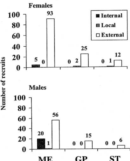
FIGURE 2. Origin of birds recruiting to three White-tailed Ptarmigan populations in Colorado. Study site abbreviations as in Figure 1. Years of study varied with site; ME: 1987–1996, GP: 1990–1996, ST: 1993–1996. Internal represents a recruit produced in that population, local recruits were produced in another study population, and external recruits came from outside the studied populations. Numbers above bars indicate sample size for recruits.
